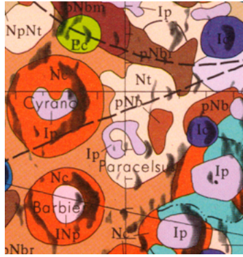
Fig. 6 Section of Geologic Map of the Central Far Side of the Moon 16 over the crater Paracelsus.
