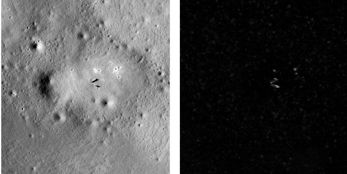
Fig. 8 Portion of vertically-flipped LRO image M118769870L centered over structures (left). North is up. Image of deviations from background model (right).
