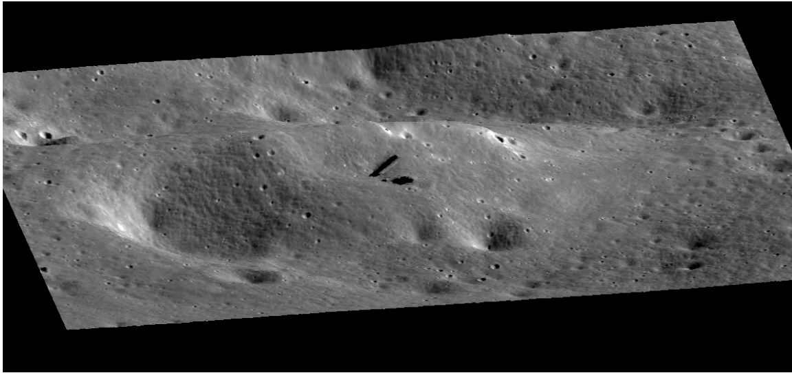
Fig. 13 Perspective view of surrounding area generated from M1153132512R. Features A and B are in the middle. The sun angle is opposite that of M118769870L.
