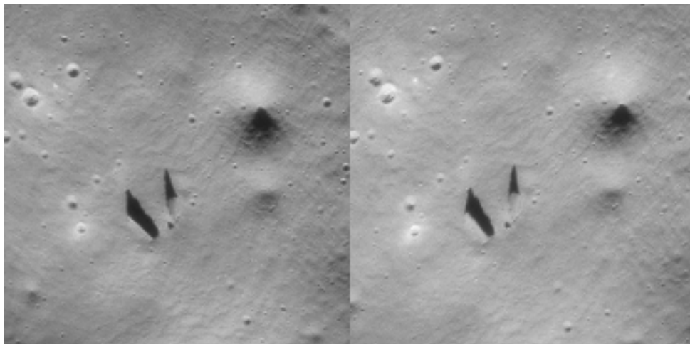
Fig. 9 Stereo pair constructed from AS15-P-8868 and AS15-P-8873. North is left. View is looking east. Notice the sun angle is similar to that in M118769870L.
